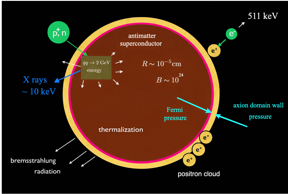
Figure 9: Summary of the structure and emission sources of an AQN. From [41].
