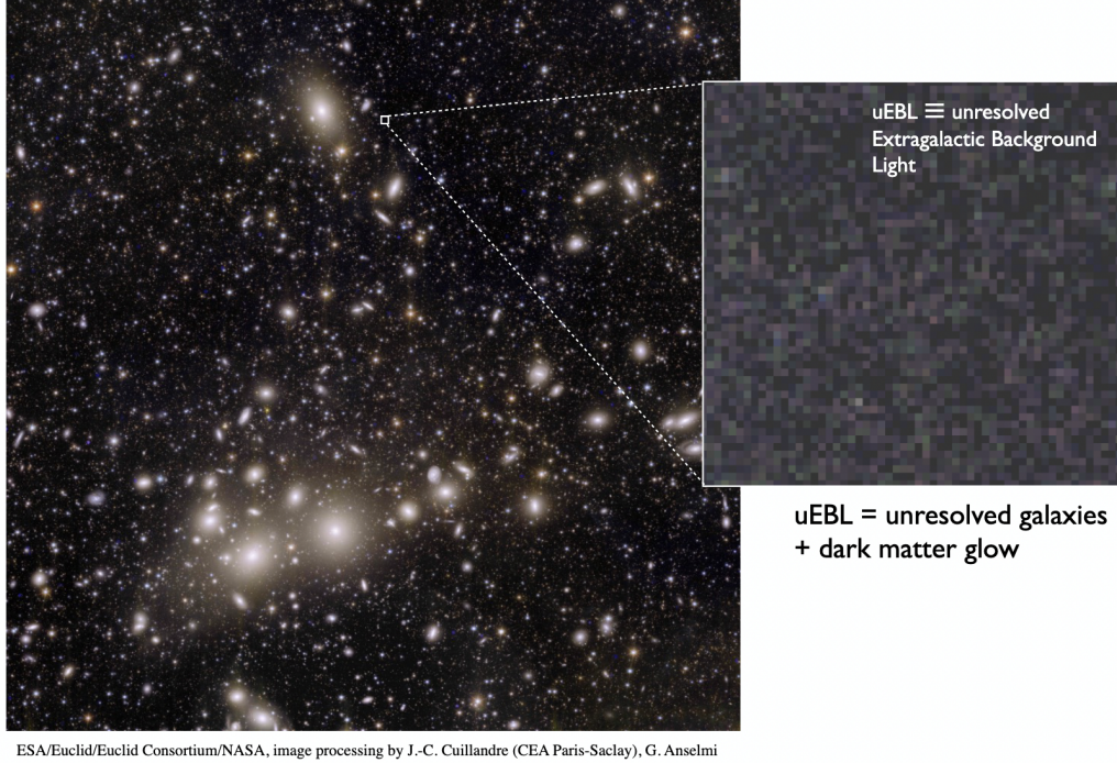
Figure 16: (Left) Euclid image of the Extragalactic Background Light (EBL). (Right) Zoom in on the unresolved EBL (uEBL), obtained after removing resolved sources. The uEBL consists of unresolved galaxies and the dark-matter glow.
