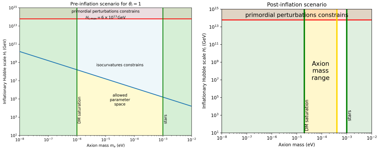
Figure 25: Inflationary Hubble scale H_I vs axion mass m_a for the pre- and post-inflation scenarios. The allowed parameter space is highlighted in yellow. Left: pre-inflation scenario (for \theta_i = 1 , \Omega_{\text{DM}} = \Omega_a ), showing constraints on H_I from isocurvature observations, DM saturation and stellar energy loss arguments. Right: post-inflation scenario with its narrow axion mass range.
