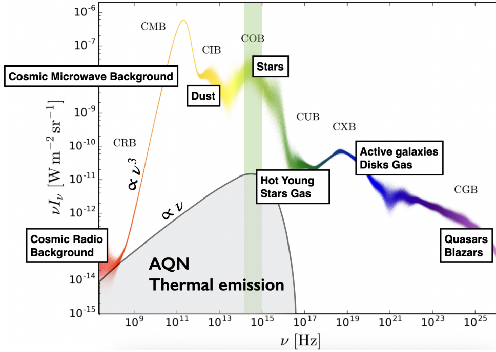
Figure 11: Comparison of the AQN thermal emission calculated for \langle m_{\text{AQN}} \rangle = 100 \text{ g} to the sky monopole calculated by [15].
