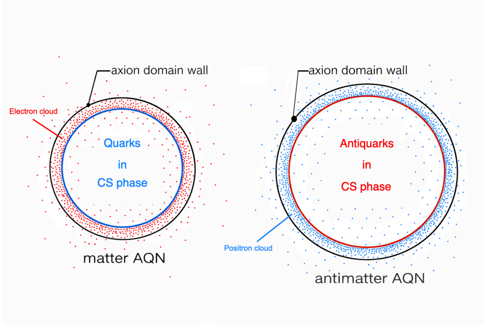
Figure 7: The quarks (antiquarks) in an AQN core are bound by an axion domain wall and stabilised by a superconducting energy gap, \Delta_{\text{gap}} \sim 100 \text{ MeV} . Matter AQNs are surrounded by an electron cloud. Antimatter AQNs are composed of an antiquark core surrounded by a positron cloud. The cosmological distribution of matter and antimatter AQNs is asymmetric (see 4.2).
