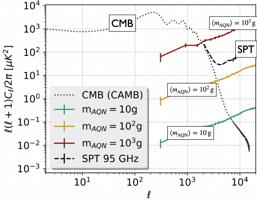
Figure 12: A \bar{Q} N emission fluctuations compared to the South Pole Telescope measurements for various values of the mean A \bar{Q} N mass [43].
