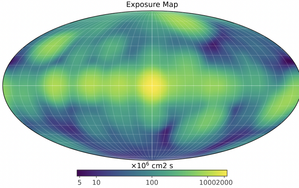
Figure 15: Exposure map for the 511 keV line observations with INTEGRAL/SPI over 20 years in Galactic coordinates. Image adapted from www.aanda.org/articles/aa/pdf/2025/10/aa55895-25.pdf .
