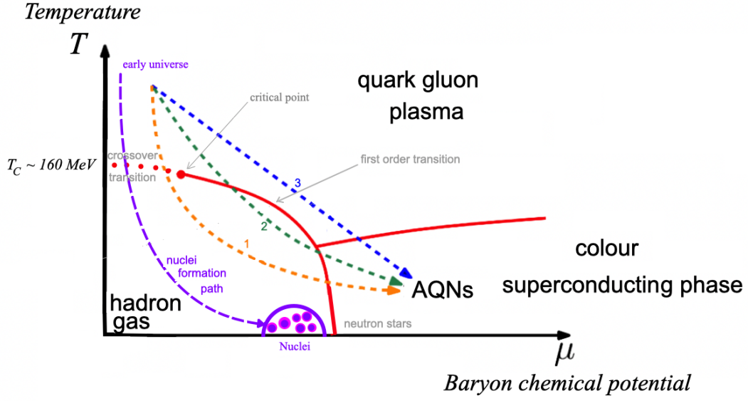
Figure 19: The QCD phase diagram and its three phases: quark-gluon plasma, hadron gas and colour superconductor. Possible formation pathways for AQNs are numbered 1,2,3. The nuclei formation pathway (dashed purple line) passes through the crossover transition and proceeds within the hadron gas phase. Adapted from [82]
