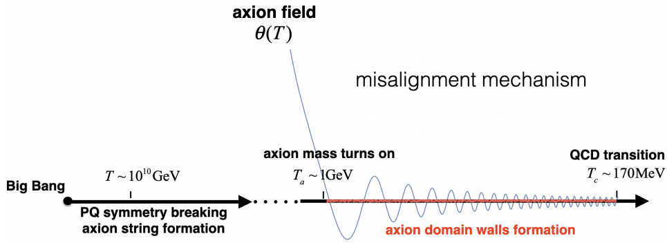
Figure 23: Timeline of axion formation from the Big Bang to the QCD transition.
