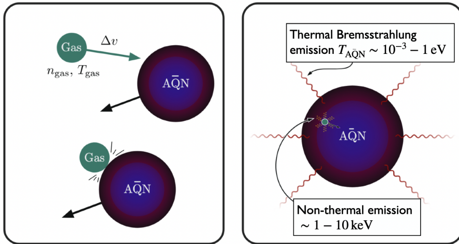
Figure 8: Left: A baryon (i.e. proton) collides with an A\bar{Q}N [not to scale]. Right: The matter-antimatter annihilation emits \sim 2 GeV of energy in the form of thermal Bremsstrahlung and a secondary beam in the 1-10 keV range [40].
