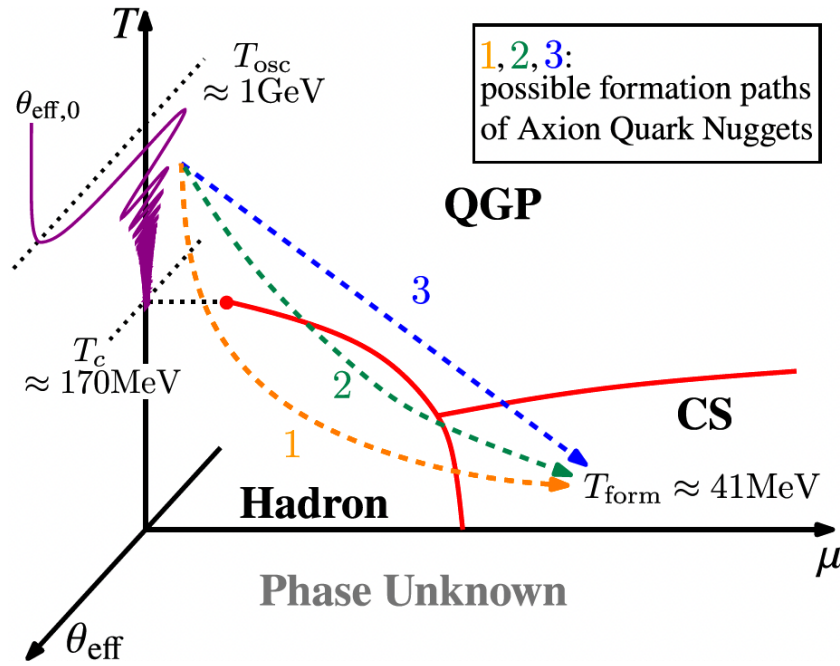
Figure 20: The oscillations of \theta_{\text{eff}} between T \sim 1 \text{ GeV} and T \sim 170 \text{ MeV} and three possible AQN formation pathways. The AQNs condensation starts around 200 MeV in the quark-gluon phase (QGP). The baryon number of the aggregates grows as they migrate through the diagram. The AQNs formation is complete \sim 41 \text{ MeV} . From [82]
