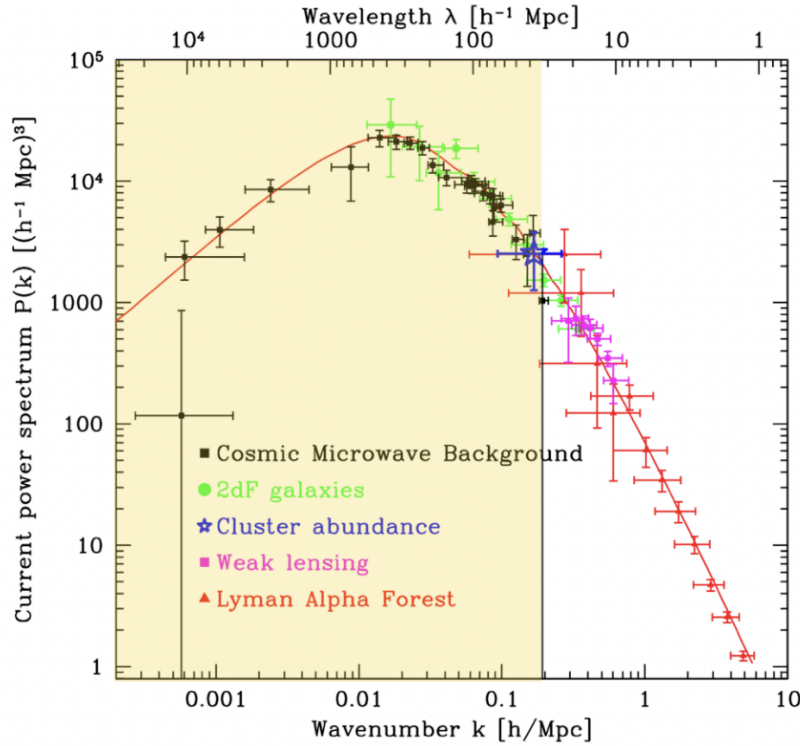
Figure 4: Power spectrum from a combination of observational probes, by [17]. The red line shows the CDM power spectrum fitted to the multiple datasets.
