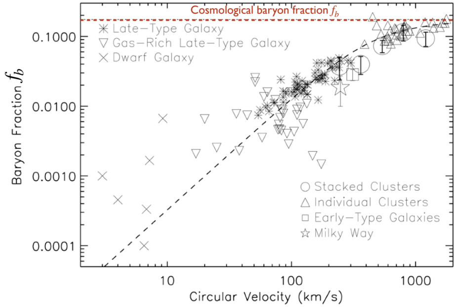
Figure 2: Fraction of baryon mass relative to total mass (circular velocity) in various systems and environments (from [13]).
