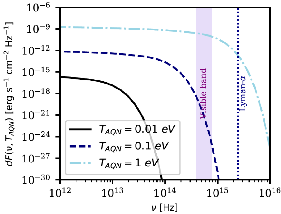
Figure 10: AQN thermal emission spectrum for various temperatures of the aggregates. The purple vertical band indicates the visible spectrum range and the Lyman- \alpha line corresponds to 10.2 eV.
