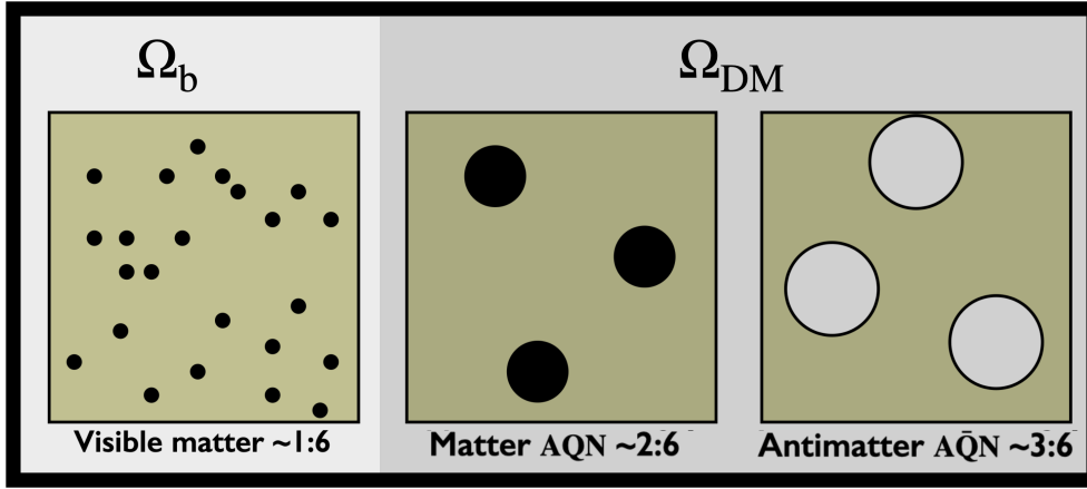
Figure 21: Visible matter, AQNs and antimatter AQNs before BBN. The aggregates form in a roughly 2:3 ratio because the axion-induced CP violation at the QCD epoch biases quark versus antiquark capture during formation, sequestering more antibaryon number in antimatter AQNs and thereby producing the observed visible baryon excess.
