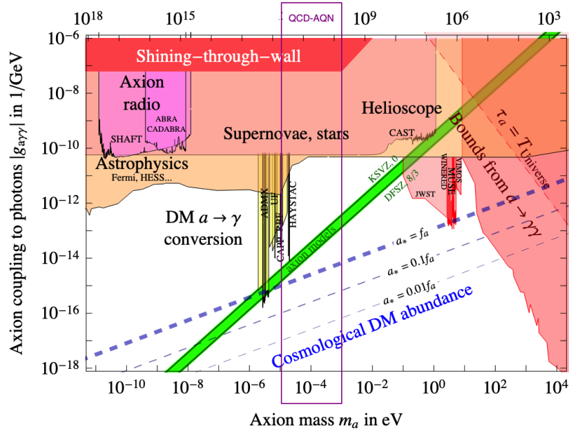
Figure 24: Parameter space for the experimental axion search. Shown are: the range favoured by axion models (green band); the initial axion vacuum expectation value a_* that reproduces the observed DM abundance (blue dashed lines); the exclusion bounds from non-observation of axion decays (coloured regions). The search window compatible with the QCD-AQN framework is the purple rectangle. Adapted from [6]
