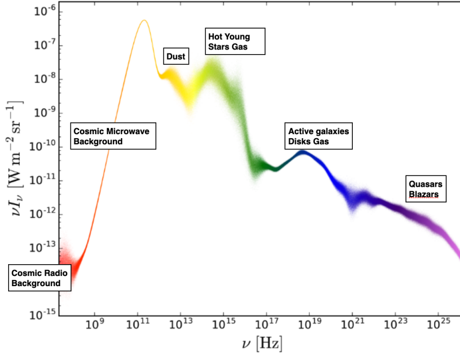
Figure 3: Intensity of the sky monopole as a function frequency [15]. The width of scattered points along the vertical direction indicate the measurement errors.
