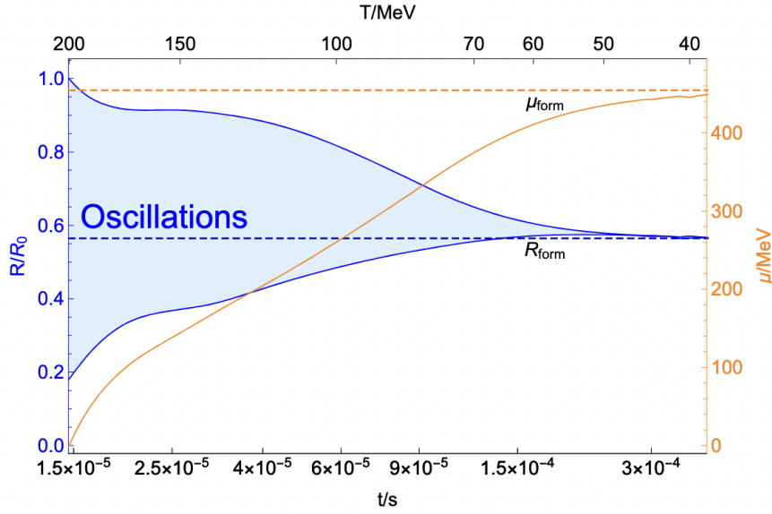
Figure 22: Evolution of the AQN radius, expressed as a fraction of the initial radius R_0 , between 200 MeV and 40 MeV. Matter AQNs and antimatter AQNs complete their formation at \sim 40 MeV. The solid orange line represents the lower envelope of the \mu oscillation. It reaches \mu_{\text{form}} \sim 450 MeV, consistent with formation of a CS phase[98, 99].
