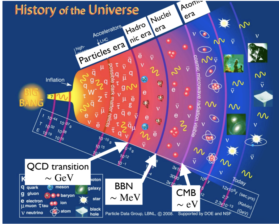
Figure 18: History of the Universe (from Particle Data Group, 2008)), annotated to highlight QCD transition, BBN and CMB.
