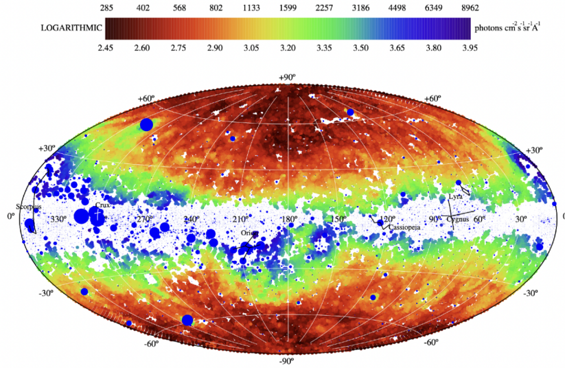
Figure 13: FUV galactic background map measured by GALEX (from [47]). Notice the isotropic excess at the galactic poles.
